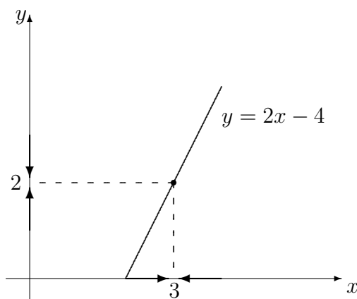
FIGURE 4.14 – La courbe y = 2x - 4 .
