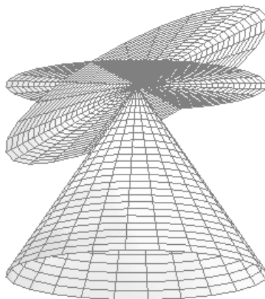
FIGURE 10.6 – Plans tangents au pic du cône z = 2 - \sqrt{x^2 + y^2} .
